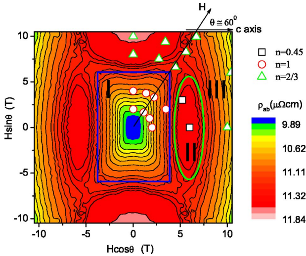
FIG. 1. (Color online) A contour plot of the in-plane resistivity \rho_{ab} of CeCoIn 5 in the H \cos \theta - H \sin \theta plane. Three different regions are found in the contour plot, which are distinguished by different values of the exponent n of the power-law T dependence of the resistivity; i.e., \rho_{ab} = \rho_0 + AT^n . The x axis of this plot is along the c axis of CeCoIn 5 and \theta_c is the angle between the diagonal of the rectangle in region I and the x axis ( c axis).
